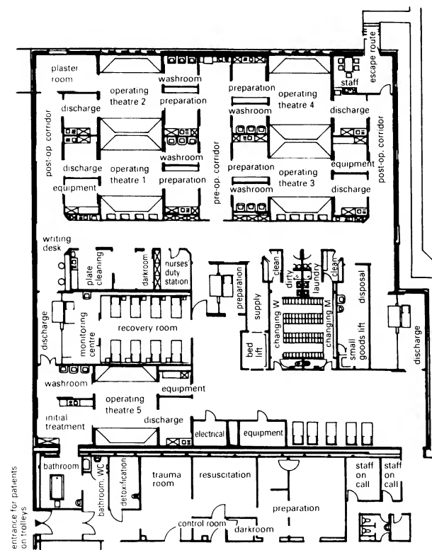
2 Ground plan of central surgical area Architects: Heinle, Wischer and Partners
